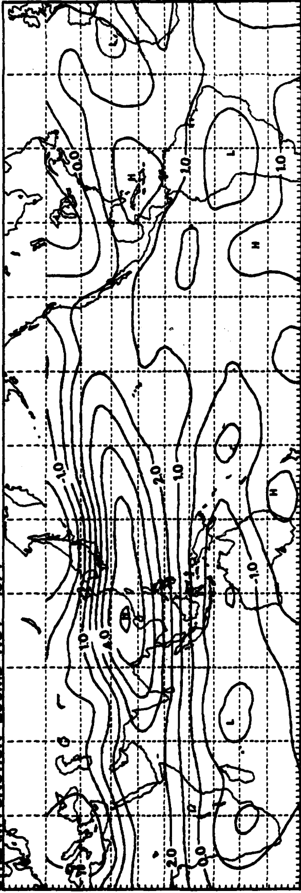
STREAM FUNCTION 200MB NOV 1974
